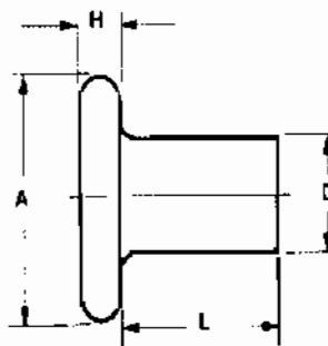
Fig. (7) : Rivet dimensions for flat head rivets in a butt joint.
