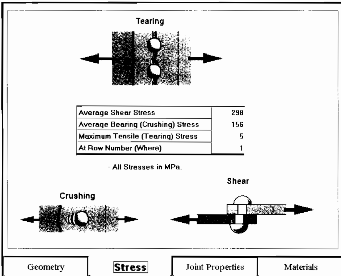
Fig. (6a) : Summary of stresses.
